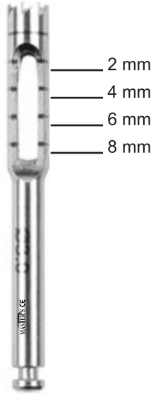
OUT \varnothing 3mm IN \varnothing 2mm 2045
